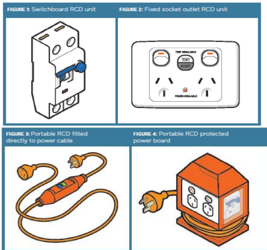
Image 1: Examples of fixed and portable RCDs. For additional information, please see the Safe Work Australia document ' Code of Practice: Managing Electrical Risks in the Workplace ' (2016).
